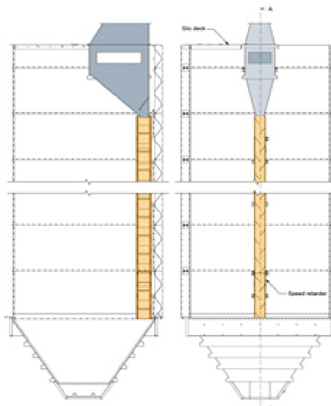
Cascade with dosing bin
